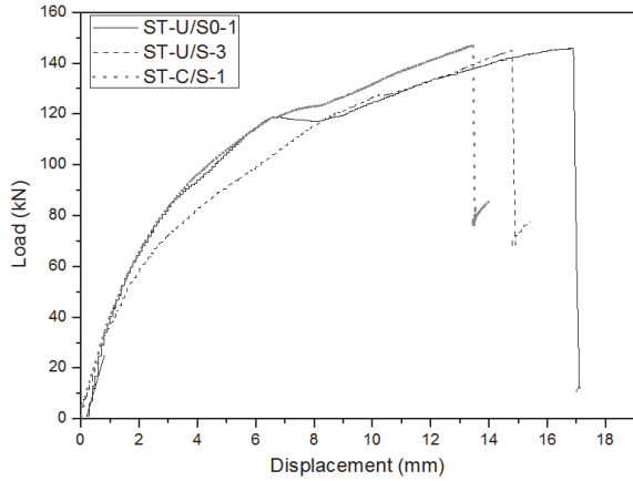
Fig. 11. Load-displacement curve
