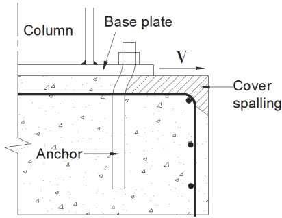
Fig. 15. Anchor bending due to cover spalling
