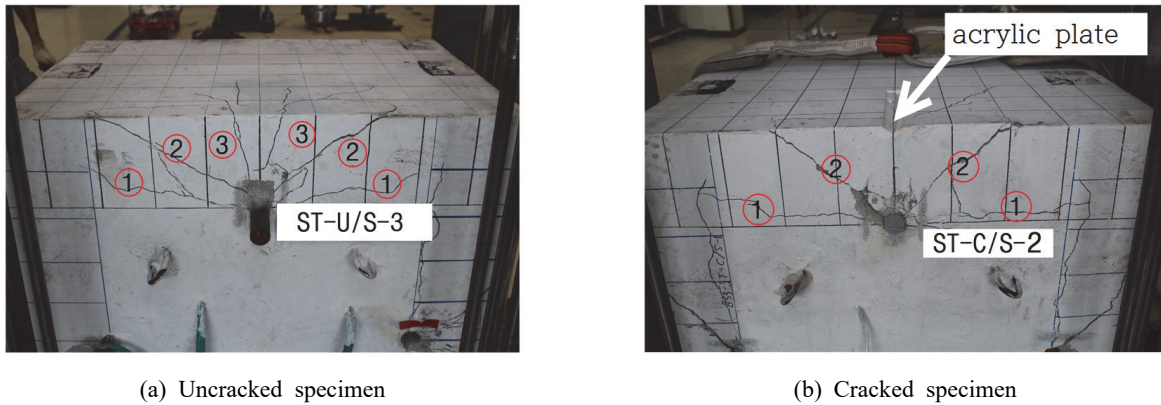
Fig. 10. Fracture shape
