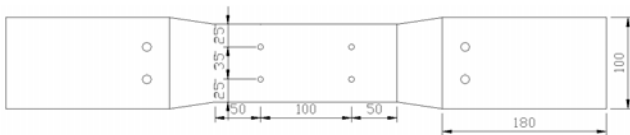
(a) Normal arrangement specimen
