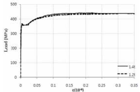
Fig. 9 Stress and strain curve of the plate
