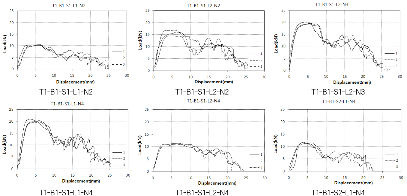
Fig. 10 Load-deflection curves
