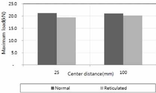
Fig. 14 Maximum forces by variation of center distances
