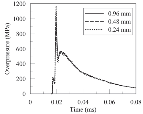
Fig. 11. Reflected overpressure histories calculated using AUTODYN for detonation of 50/50 Pentolite of 1kg at Z = 0.12\text{m/kg}^{1/3}
