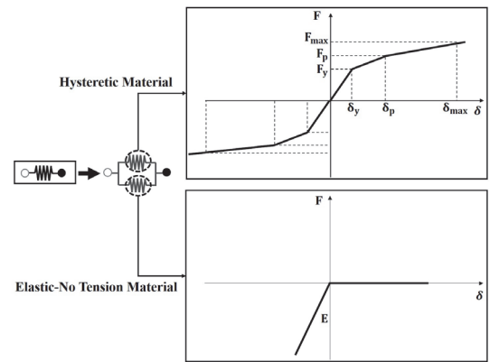
Fig. 8. Spring elements for angles and gap opening
