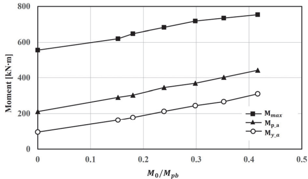
Fig. 11. Moment according to the decompression moment
