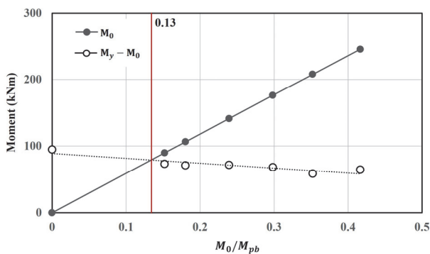
Fig. 13. Self-centering capacity
