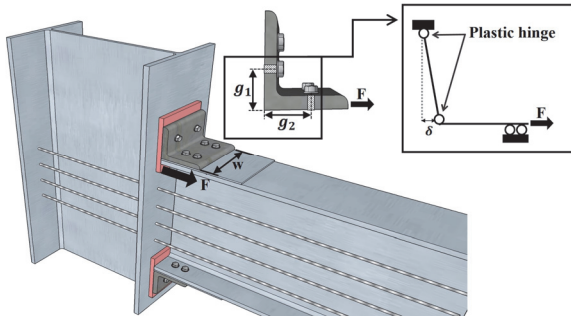
Fig. 3. Angle analytical model in self-centering connection
