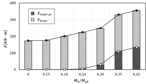
Fig. 14. Energy absorption
