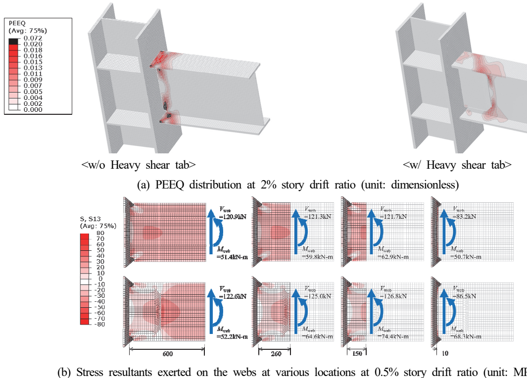
Fig. 11. Comparison of PEEQ and internal forces based on numerical analysis
