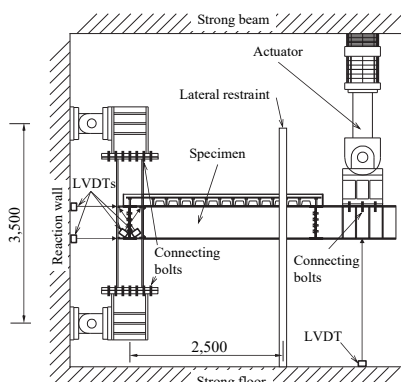
Fig. 3. Test set-up
